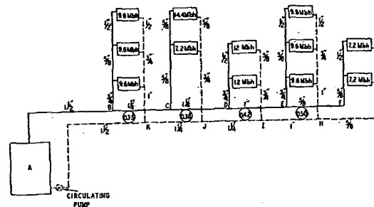
FIG. 5. A FORCED CIRCULATION DIRECT RETURN SYSTEM
