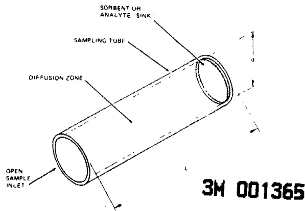
Figure 1 A simple tube-type diffusion sampler.
