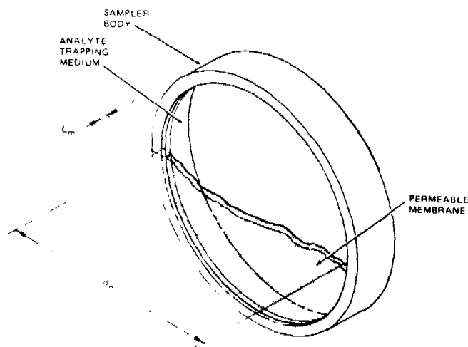
Figure 2 A typical membrane-type permeation sampler.
