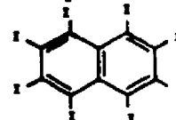
Polychlorinated Naphthalenes
