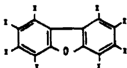
Chlorinated Dibenzofurans
