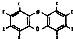
Chlorinated Dibenzodioxin
