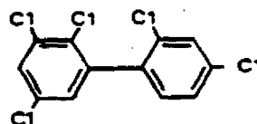
2,2',3,4',5-pentachlorobiphenyl
