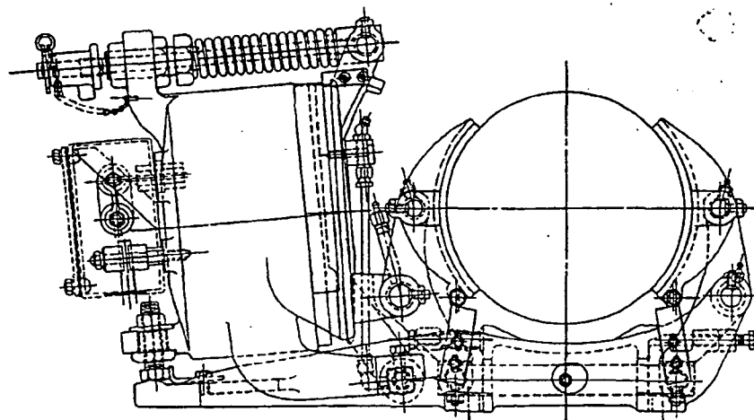
GENERAL ARRANGEMENT FOR S.M. DES. DRG. 71045
