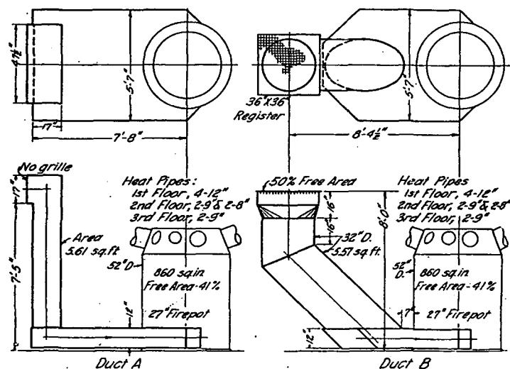
FIG. 6. TWO TYPES OF RECIRCULATING DUCT TESTED
