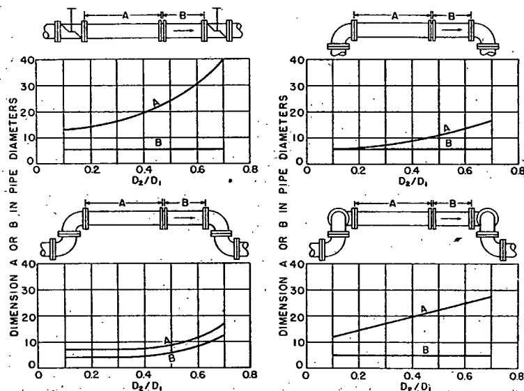
FIG. 23. MINIMUM CONDITIONS TO BE OBSERVED WHEN INSTALLING ORIFICES AND NOZZLES BETWEEN FITTINGS AND VALVES
