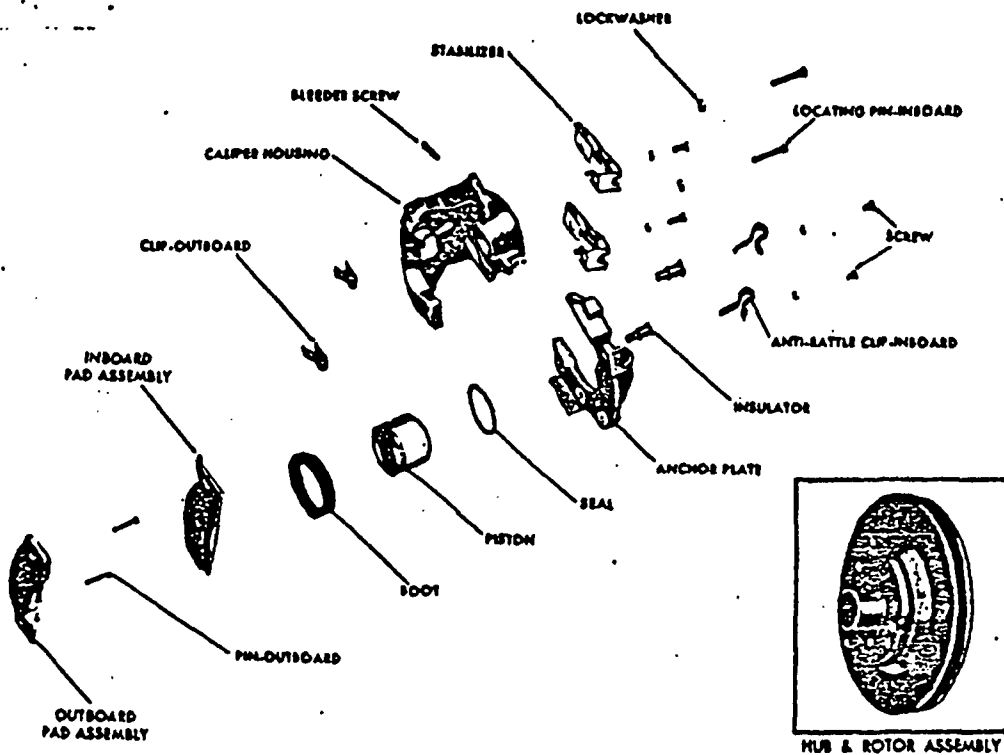
1973-70 KELSEY-HAYES SINGLE PISTON DISC BRAKE — FORD
