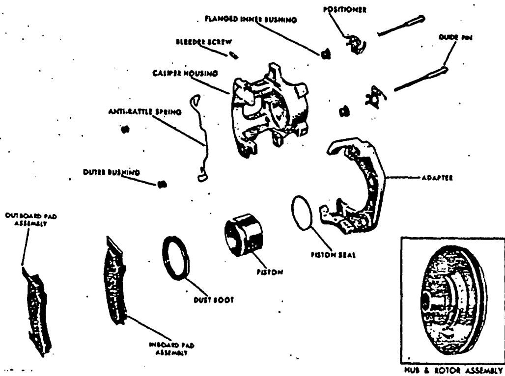
1973-70 KELSEY-HAYES SINGLE PISTON DISC BRAKE—CHRYSLER
