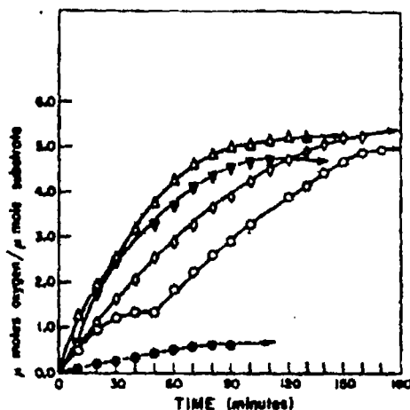
FIG. 3. Rates of oxygen uptake by washed cell suspensions of biphenyl-grown Achromobacter BP cometabolizing various substrates. All rates are corrected for endogenous respiration. (○), p -Chlorobiphenyl; (Δ), m -chlorobiphenyl; (○), o -chlorobiphenyl; (○), m -chlorobiphenyl; (▽), 4,4'-dichlorobiphenyl; (●), 2,2'-dichlorobiphenyl.
