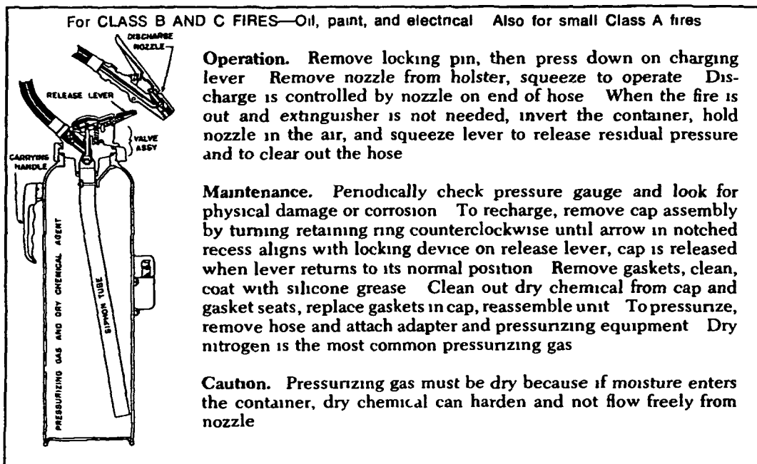
FIG 43-22 —Dry-chemical fire extinguisher, stored pressure type (Style discontinued in 1974)
