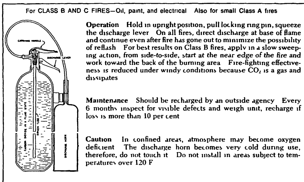
FIG 43-23 —Carbon dioxide fire extinguisher
