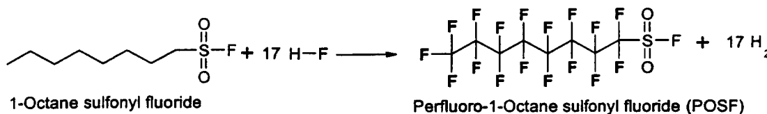
Figure 3.2. Example of the ECF process
