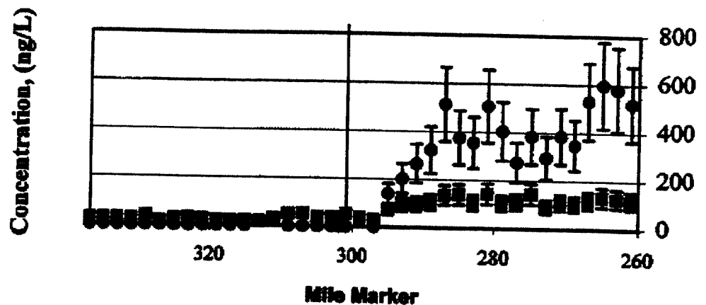
Figure 5.4 PFOS and PFOA Levels in the Tennessee River. The line at 301 mile indicates the location of the incoming effluent from the fluorochemical manufacturing plant (Hansen et al., 2002).
