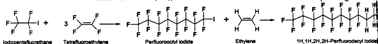
Figure 3.4. Example of the telomerisation process
