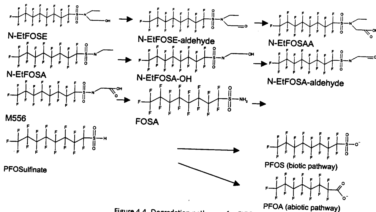
Figure 4.4. Degradation pathway of n-EtFOSE to PFOS and PFOA (3M, 2000b, 3M, 2001e).
