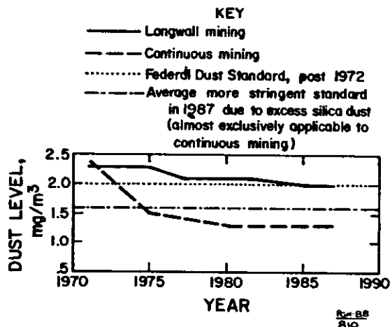
Figure 1. Average dust levels of operator samples from selected underground mining methods.
