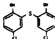
FENTICLOR 2,2'-Thio-bis(4-chlorophenol)
