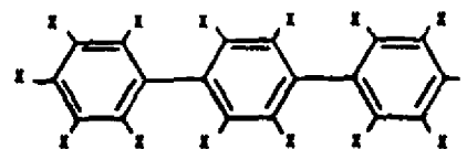
Polychlorinated Terphenyls
