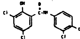
3,3',4,5'-Tetrachlorosalicylanilide (TCC)
