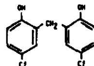
DECACHLOROPHENE 2,2'-Methylene-bis(4-chlorophenol)
