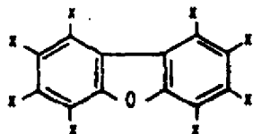
Chlorinated Dibenzofurans
