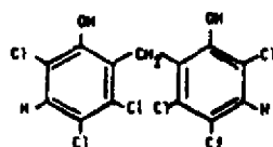
HEXACHLOROPHENE 2,2'-Methylene-bis(3,4,6-trichlorophenol)
