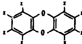
Chlorinated Dibenzodioxin
