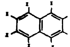
Polychlorinated Naphthalenes
