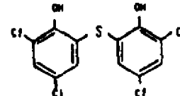
DITHIONOL 2,2'-Thio-bis(4,6-dichlorophenol)
