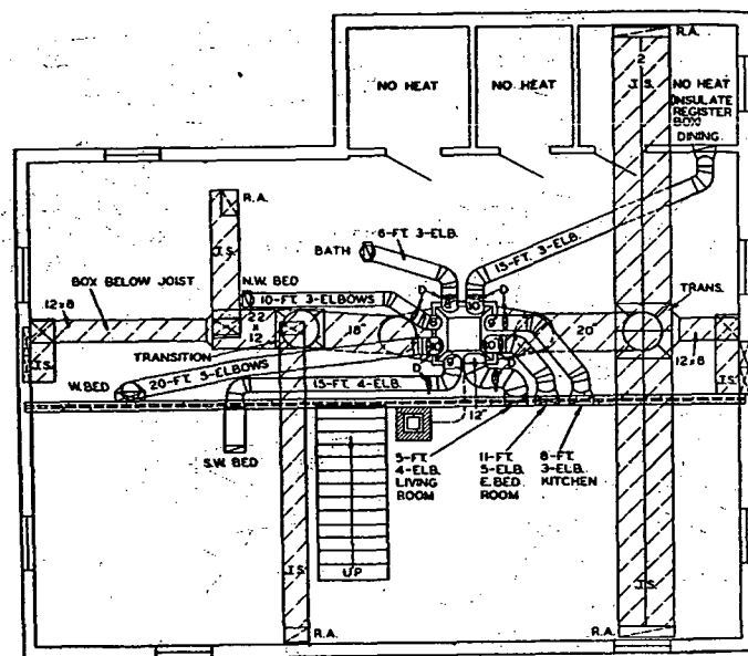
FIG. 6. TYPICAL BASEMENT LINE DRAWING
