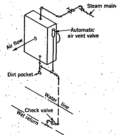
FIG. 5. UNIT HEATER CONNECTED TO ONE-PIPE AIR-VENT SYSTEM
