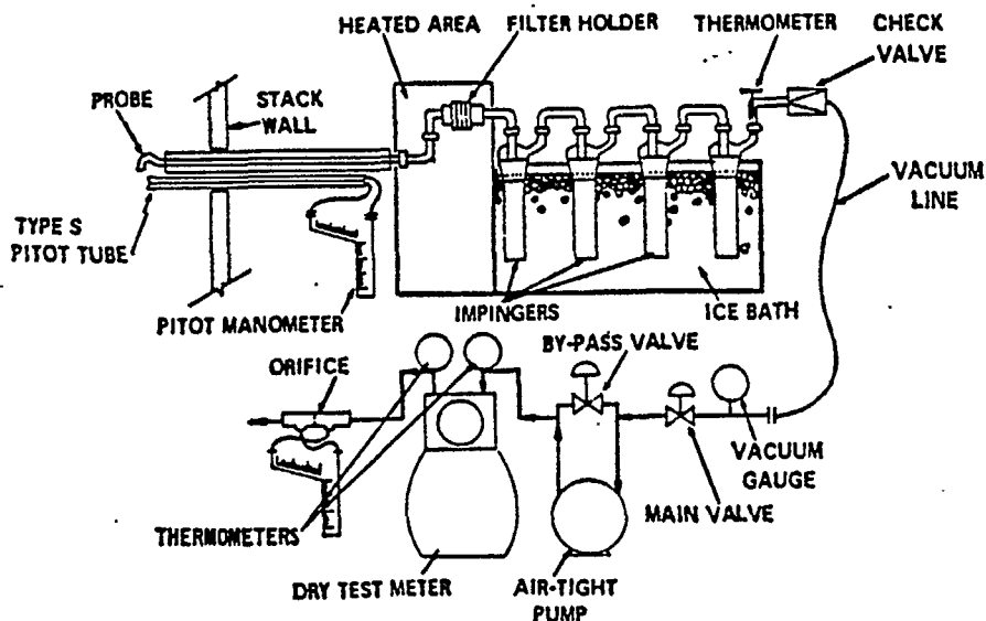
Figure 104-1. Beryllium sampling train
