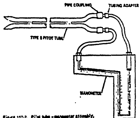
Figure 102-2. Pitot tube-manometer assembly.
