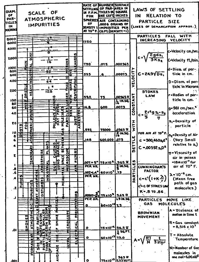
FIG. 1. SIZES AND CHARACTERISTICS OF AIRBORNE PARTICULATE MATTER
