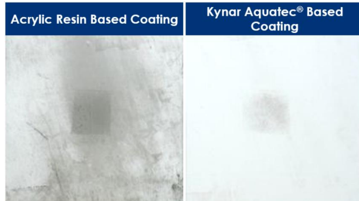
Figure 4. Dirt Pick Up Study with Acrylic-Based Resin Coating vs Kynar Aquatec® Based System
