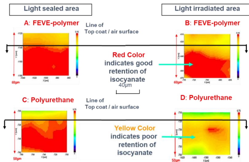
Figure 16. 15-Year Sunlight Exposure of FEVE polymer and polyurethane systems
