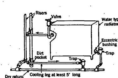
FIG. 45. TWO-PIPE TOP AND BOTTOM OPPOSITE END RADIATOR CONNECTIONS
