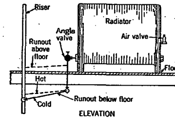
FIG. 44. ONE-PIPE RADIATOR CONNECTIONS
