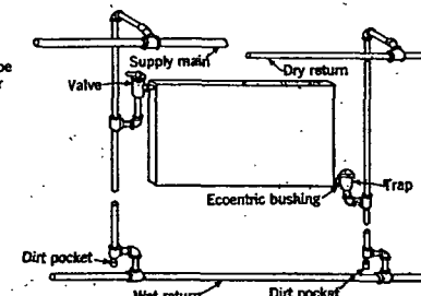
FIG. 46. TWO-PIPE CONNECTIONS TO RADIATOR HUNG ON WALL
