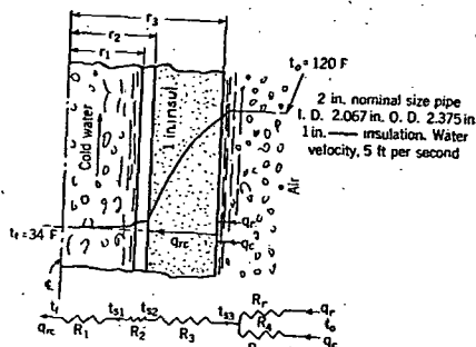
FIG. 4. HEAT TRANSFER CONDITIONS IN AN INSULATED COLD WATER LINE
