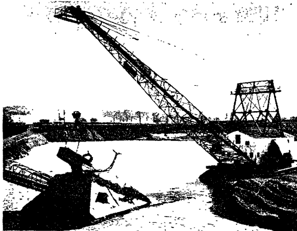
Above, left: Scene at the Radum plant: a dragline with a 10-cu.-ft. bucket charging a floating hopper. Right: A portion of the Radum plant, viewed from the control tower at the top of the main plant. Note the typical Kaiser use of conveyors.
