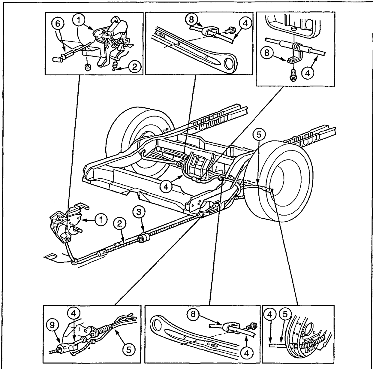
Typical Parking Brake Components
