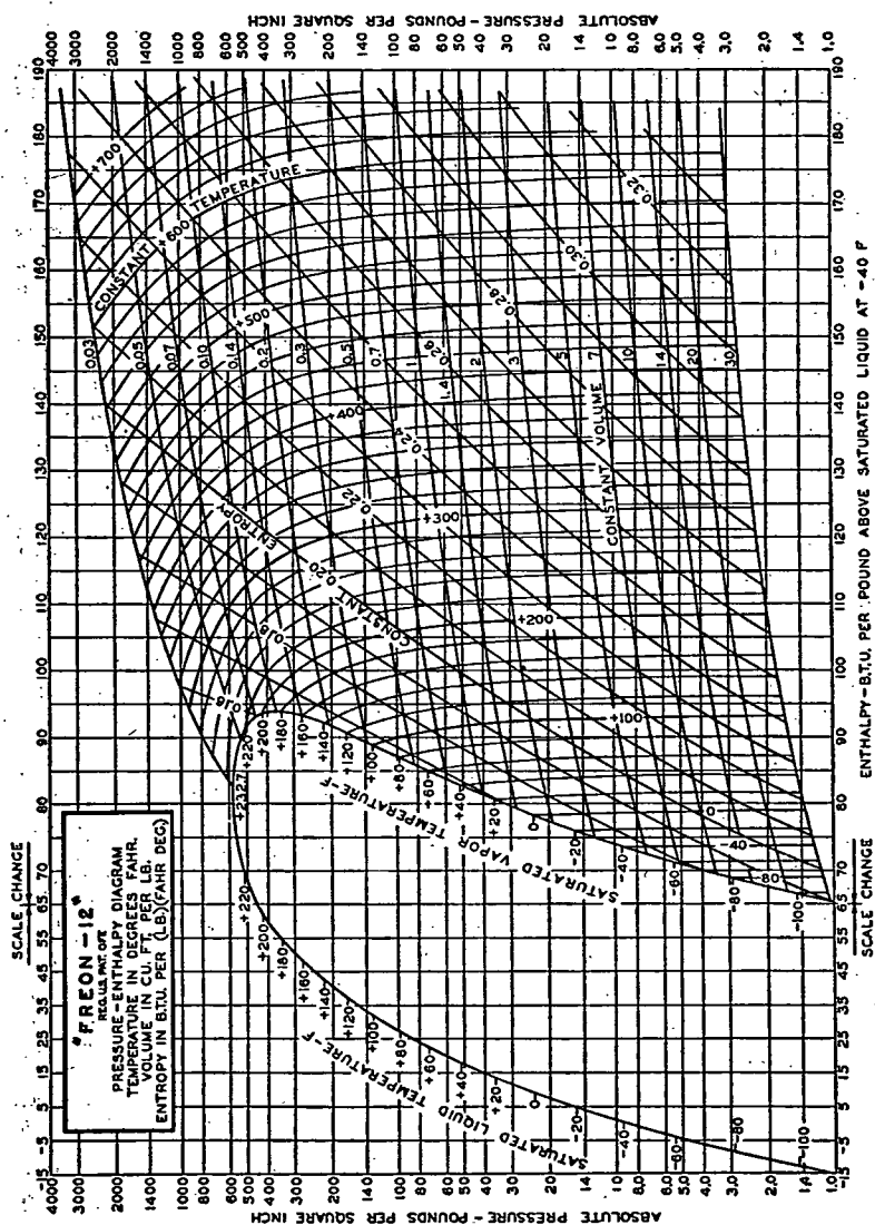
FIG. 1. PRESSURE-ENTHALPY DIAGRAM FOR FREON-12
