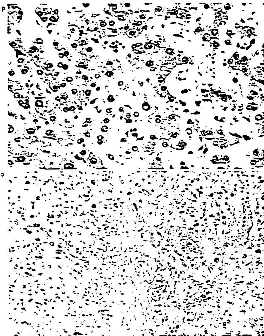
Fig. 5c. Focal portal fibrosis (left upper corner) and activated proliferating and pleomorphic sinusoidal lining cells with activated proliferating and pleomorphic sinusoidal lining cells. Trichrome (Gold-ner) stain, blue filter, x 250. d. Conspicuous focal dilatation of sinusoids. Activation and moderate polymorphism of proliferated hyperplastic sinusoidal lining cells. Enlarged hepatocytes with hyperchromatic nuclei, some of them binuclear. Potential precursor stage of angiosarcoma? Courtesy of Professor Müller-Wallat, Institute of Pathology, Årberg, H. & E. x 400
