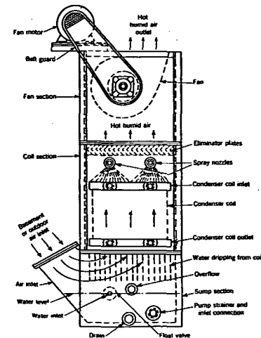
Fig. 10 Schematic View of an Evaporative Condenser
