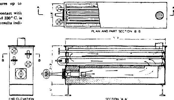
Figure 1. Heater
