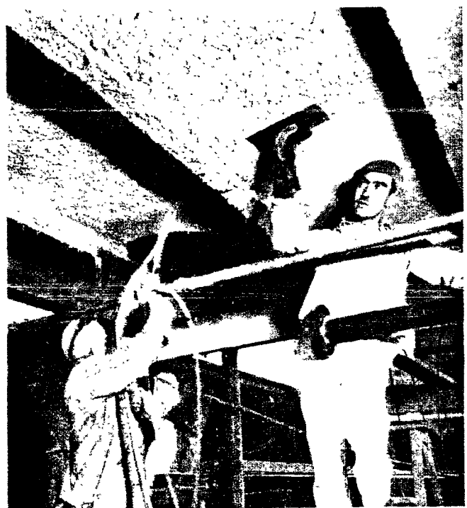
Spraying K & M Limpet as a deck insulation
