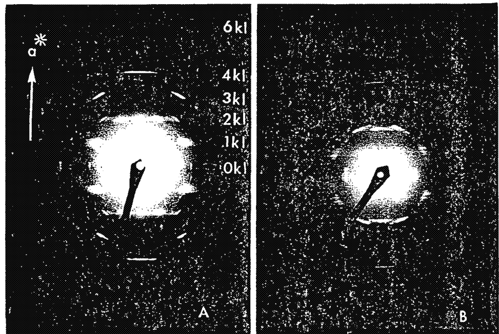
FIG. 2. Selected area electron diffraction patterns obtained on fibers of chrysotile obtained during air sampling at brake repair shops. In A, the reciprocal a^* axis is marked a^* as are the layer lines in the (0kl) series. Indexing of upper right quadrant yielded 16 reflections corresponding to single crystal X-ray diffraction analysis of Whittaker and Zussman, 1956. Pattern in (B) displays "smearing" of reflections in a "clockwise" manner suggesting interplanar rotation.
