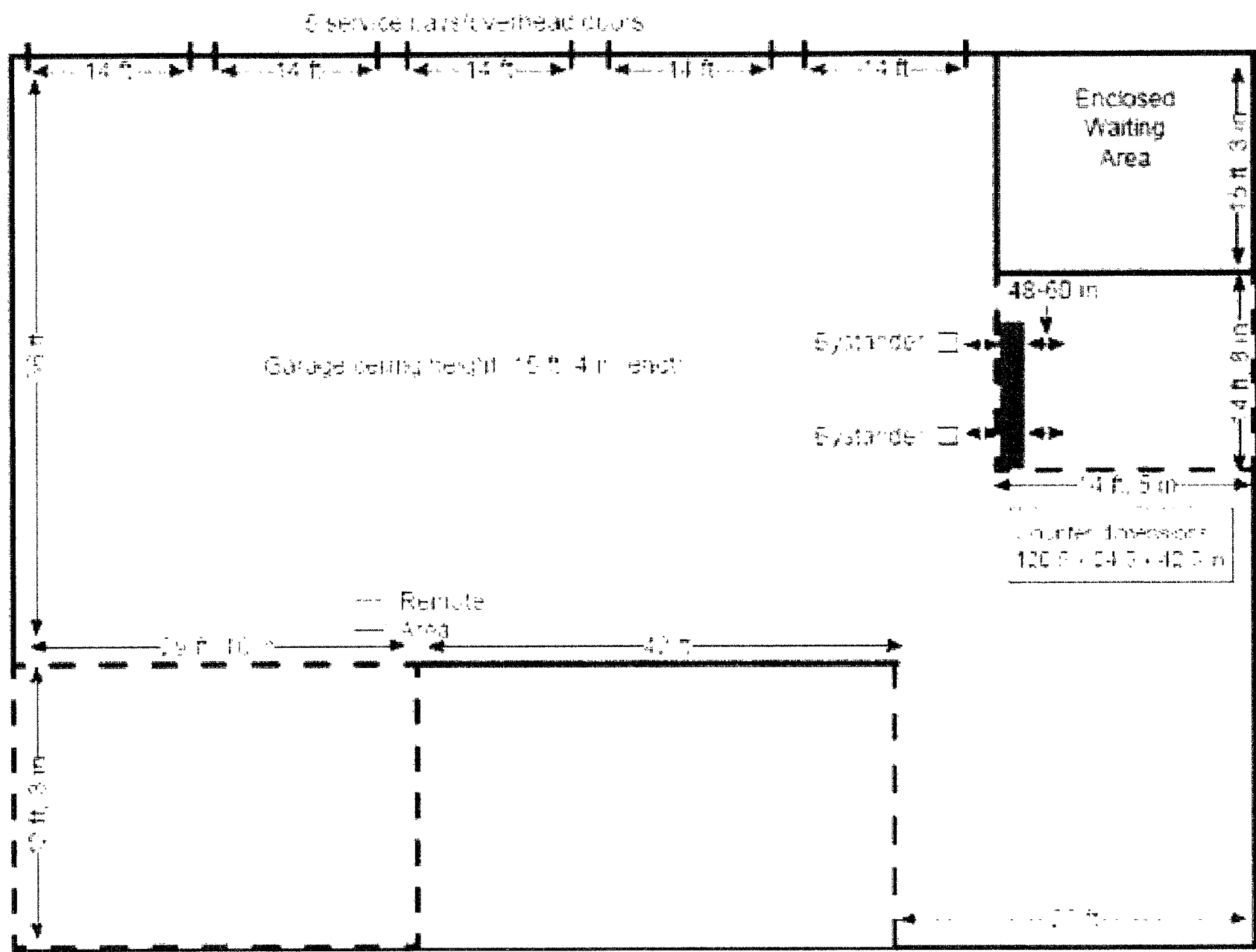
Figure 3A: Garage layout and dimensions
