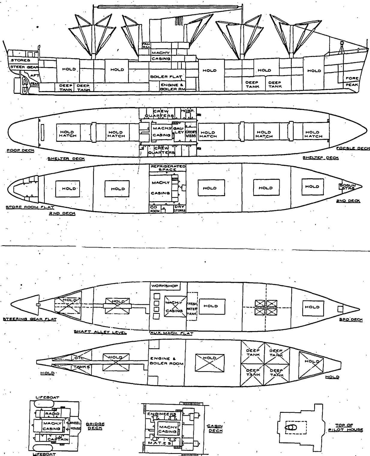
FIG. 1. ARRANGEMENT OF A TYPICAL CARGO VESSEL
