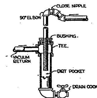
FIG. 14. DETAIL OF MAIN RETURN LIFT AT VACUUM PUMP
