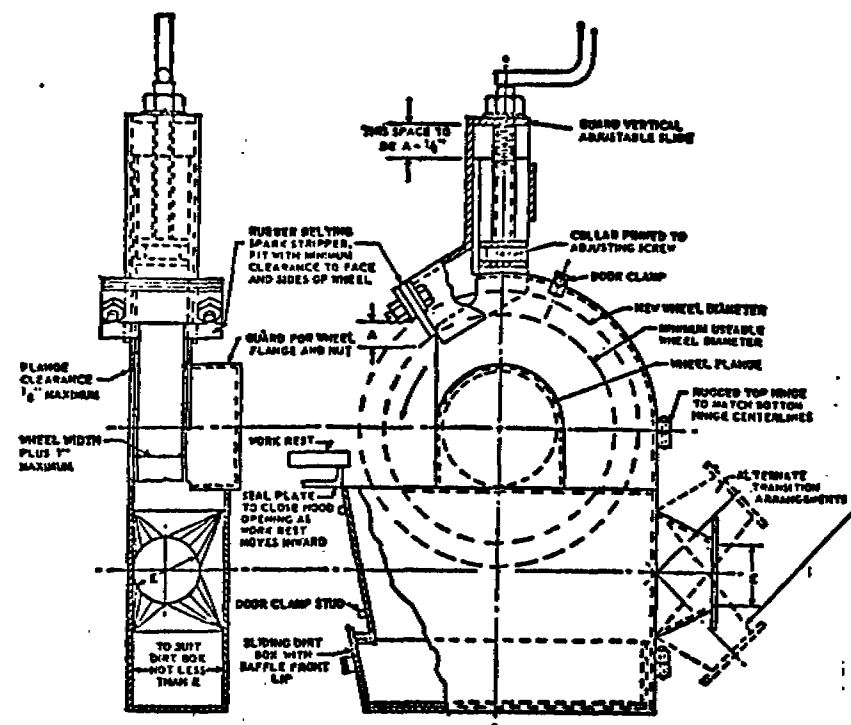
Fig. G-2 Standard Grinder Hood
