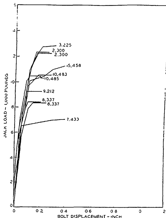
Fig. 2—Pull test performance of \frac{5}{8} -in bolt anchorage supplemented with ROC-LOC product. Compare with Figs. 3 and 4, all replicate tests.
