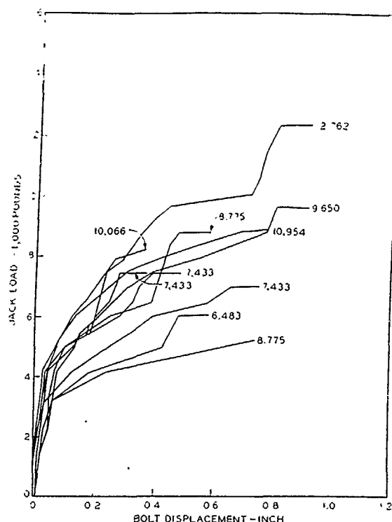
Fig. 3—This pull-test data is also for a \frac{5}{8} -in. bolt which is anchored with \frac{3}{8} -in. expansion shell only.
