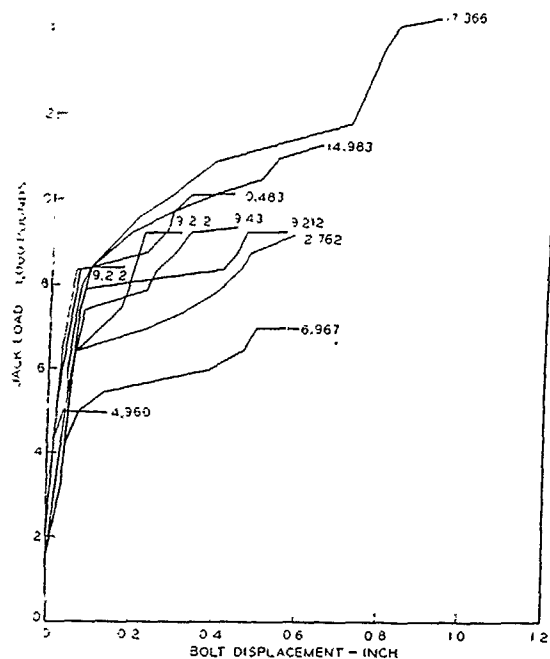
Fig. 4—This test series is of \frac{5}{8} -in. bolts using a typical epoxy resin to supplement anchorage. Tests made by U.S. Bureau of Mines.
