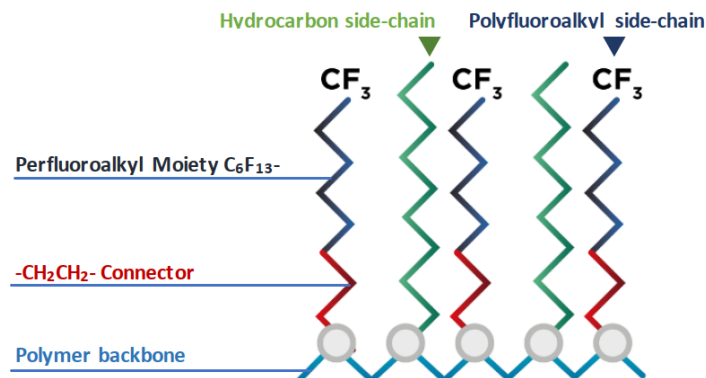
Figure 4. Side-chain fluorinated polymer structure.
