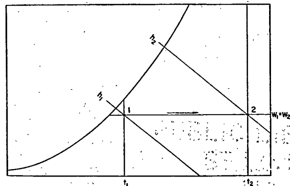
FIG. 7. SOLUTION OF EXAMPLE 3 ON A.S.H.V.E. PSYCHROMETRIC CHART
