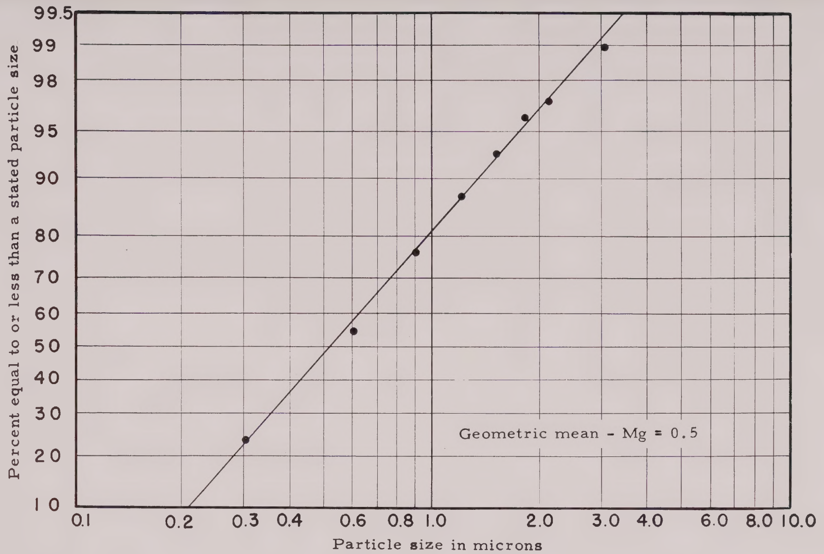
Figure 12.—Particle-size distribution of a typical air-borne foundry dust.
