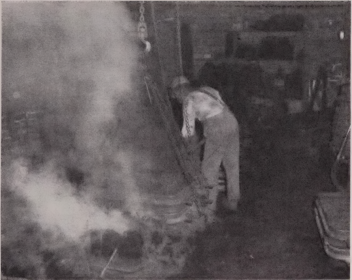
Figure 10.—Shakeout of casting from floor mold using a chain hoist.
