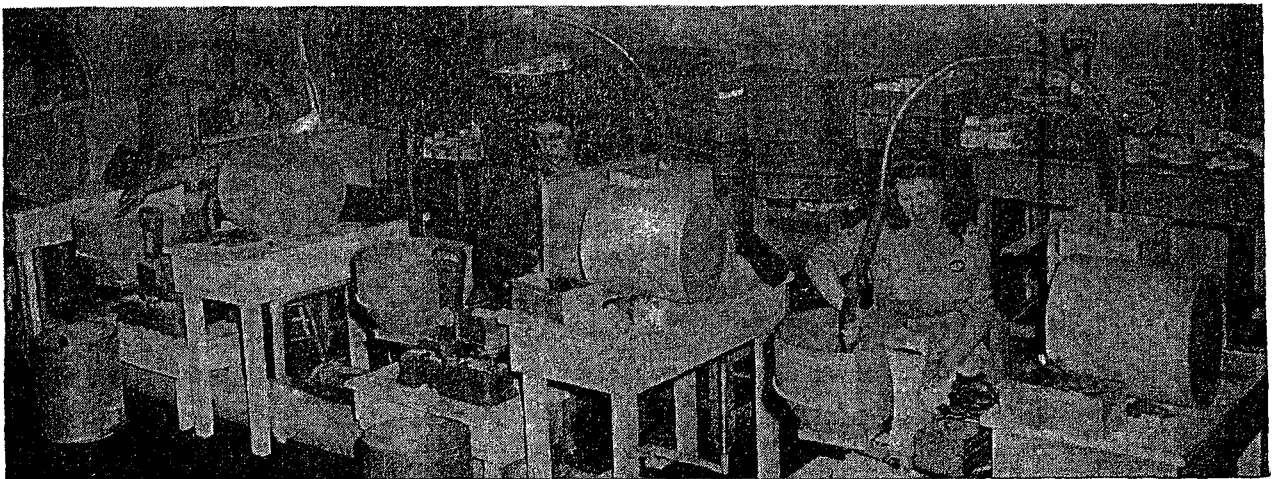
Part of packaging assembly line. Hoppers of asbestos on scales balance boxes of measured weights. As weights are removed one by one, asbestos is vacuum drawn out of hopper into cotton bag through flexible transparent tube to return scale to balance. Foot treadle controls vacuum.
