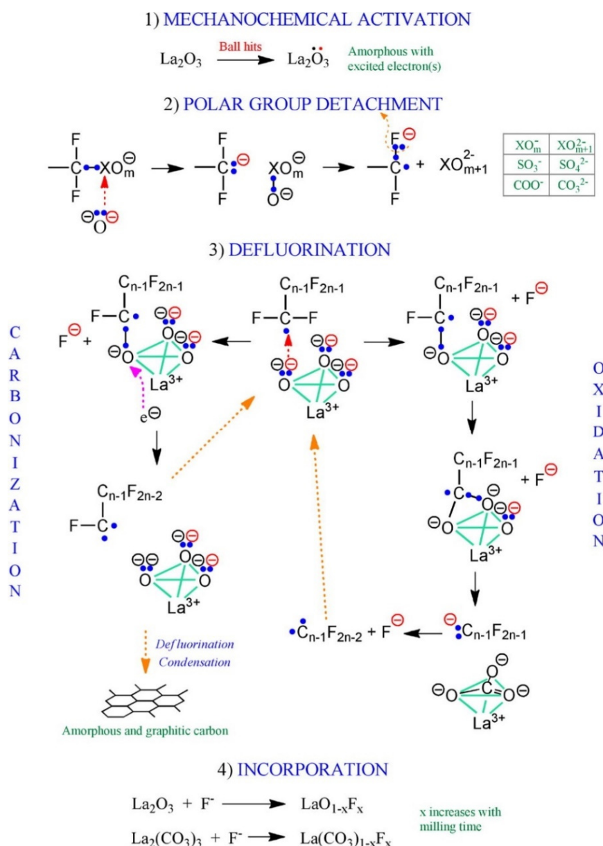
Figure 4. Proposed mechanistic pathways for the stoichiometrical activation of selected PFASs with \text{La}_2\text{O}_3 (reprint from [119], with permission from Elsevier).
