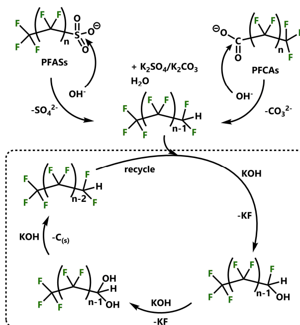
Figure 2. Proposed mechanism of reaction of KOH with PFOS and PFOA under mechanochemical treatment [114].
