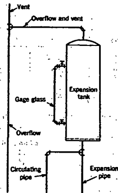
FIG. 15. AN OPEN EXPANSION TANK
