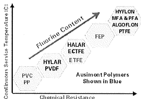
Fluoropolymer Products Service Temperature versus Chemical Resistance
