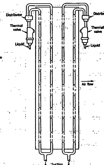
FIG. 7. ARRANGEMENT FOR DEPTH CONTROL
