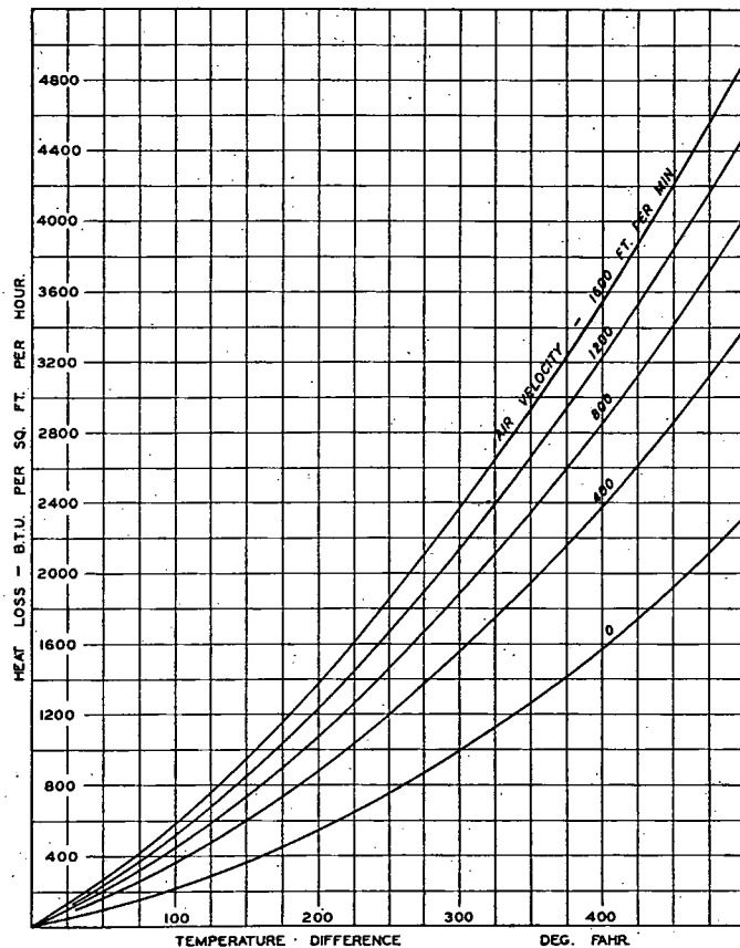
FIG. 5. HEAT LOSSES FROM SURFACES EXPOSED TO VARIOUS AIR VELOCITIES
