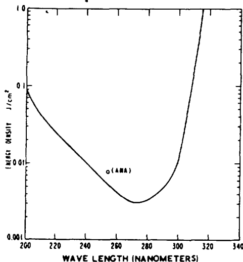
Figure 8 — Threshold Limit Values for Ultraviolet Radiation
