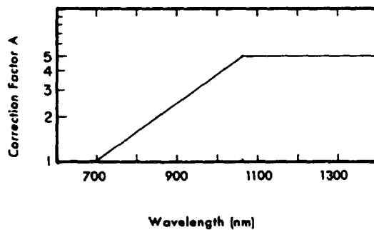
Figure 2 — TLV correction factors for laser wavelengths (eye).
