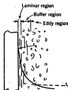
FIG. 1. THERMAL CONVECTION CONDITIONS
