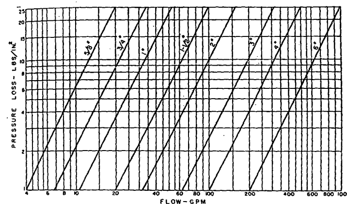
FIG. 6. PRESSURE LOSSES IN WATER METERS
