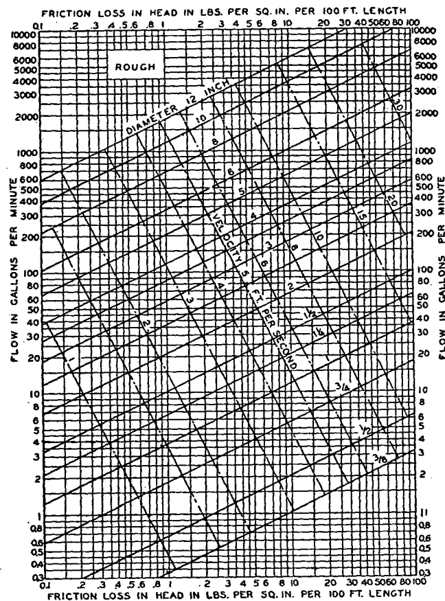
FIG. 5. FLOW CHART FOR ROUGH PIPE
