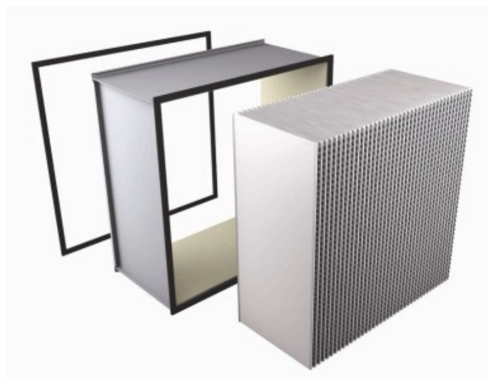
Figure 5.3: Scheme of a deep pleated HEPA filter.
