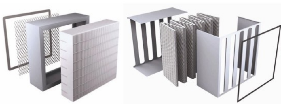
Figure 5.4: Scheme of mini-pleated HEPA filters.
