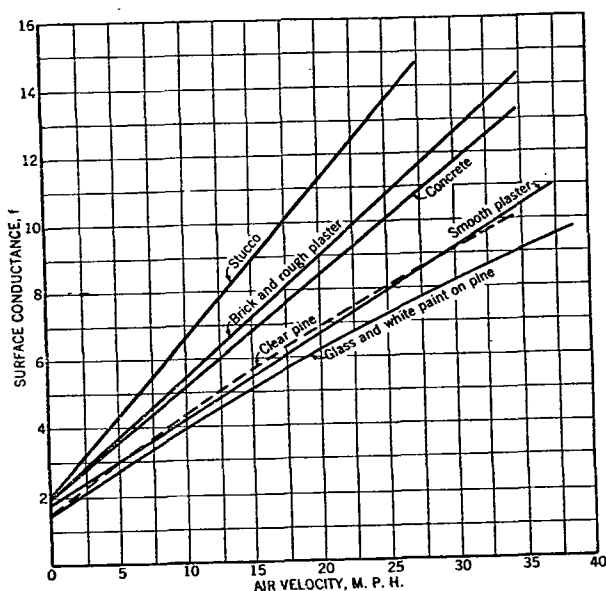
FIG. 3. CURVES SHOWING RELATION BETWEEN SURFACE CONDUCTANCES FOR DIFFERENT SURFACES AT 20 F MEAN TEMPERATURE
