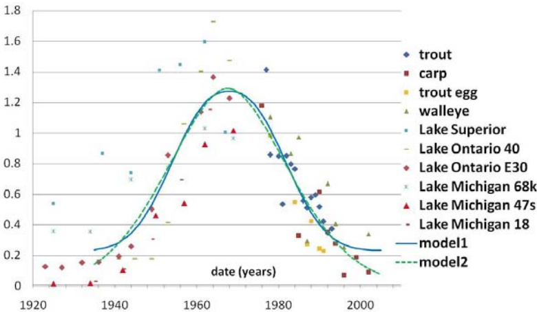
Figure 1. F(t, θ) for models with all parameters fitted without constraints (model 1) and forced to tend towards 0 (model 2).
