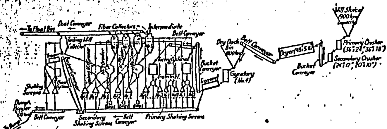
FIG. 4—Typical flow-sheet of a cross-bed process
