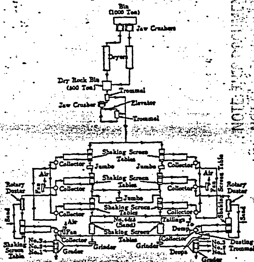
FIG. 5.—Typical flow sheet of a slip-fiber mill.
