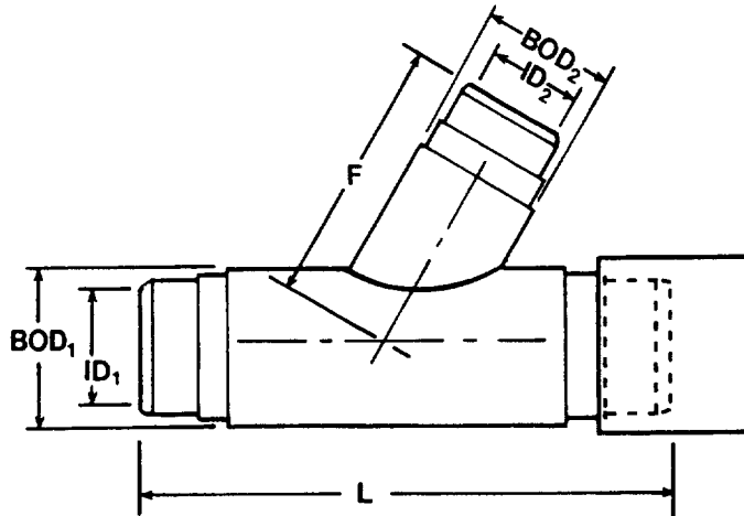
BRANCH PIPE LAYING LENGTH (F DIMENSION)
