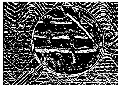
Magnified Section of "Loaded" AIR-MAZE Air Filter Element. Note that dust has been quite evenly impinged on the wires. No obstructed spaces can be seen. This feature accounts for the Low Pressure Drop and Non-clogging characteristics of AIR-MAZE.
